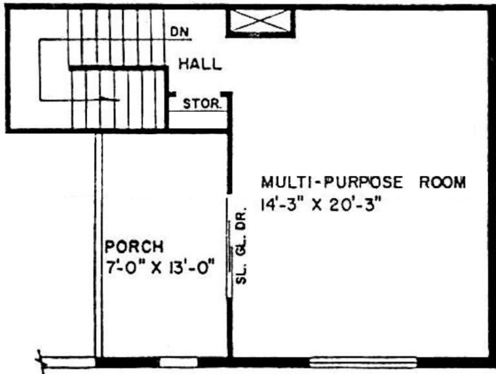
M-5 SECOND STORY REVERSE
