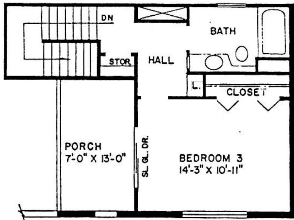
PLAN M-5 SECOND STORY
