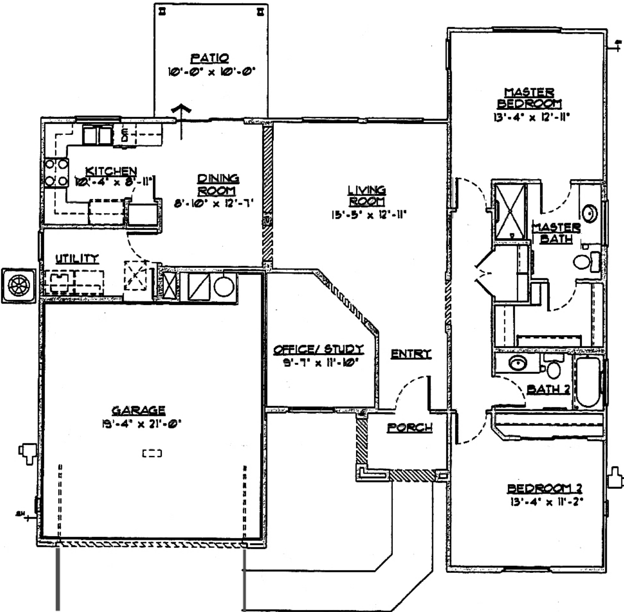
THE "HERITAGE" 9223
