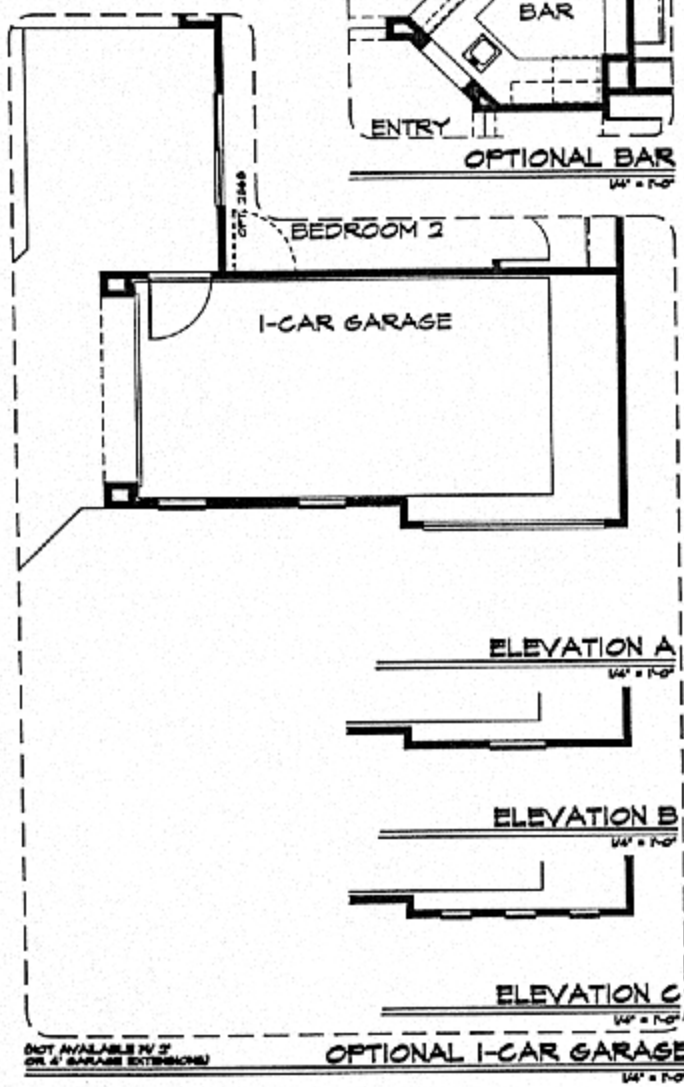
FLOOR PLAN - 9137 OPTIONS 1/4" = 1'-0"
