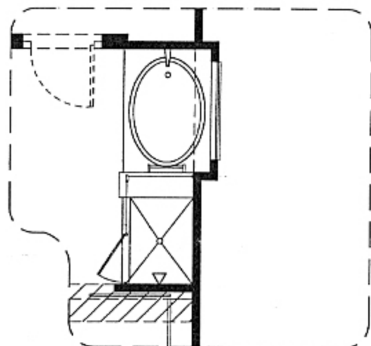
OPT. SEP. TUB & SHOWER 1/4" = 1'-0"
