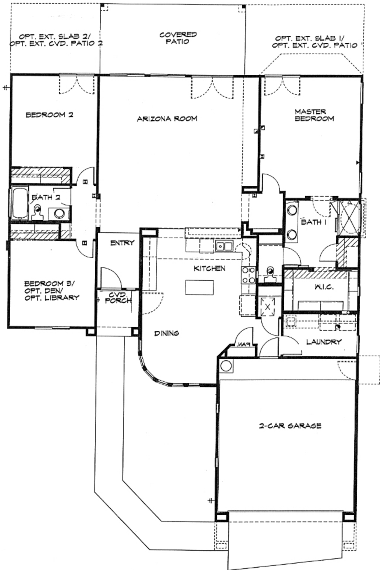
FLOOR PLAN - 9136
