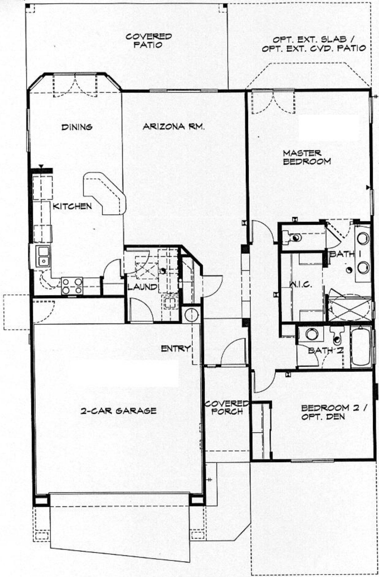
FLOOR PLAN - 9028 1/4" = 1'-0"
